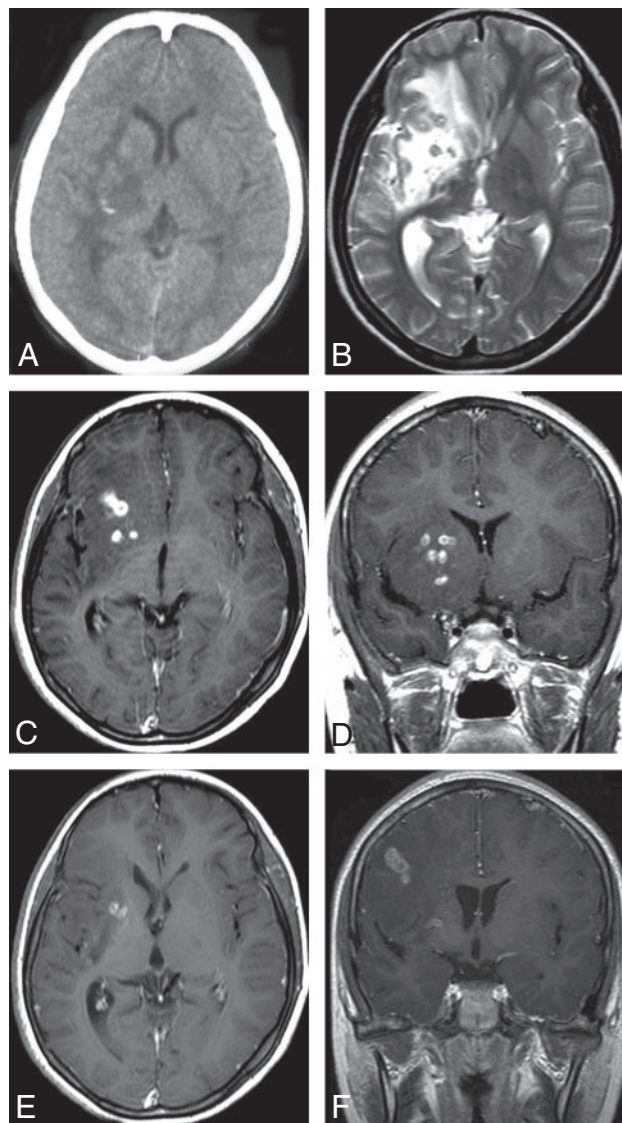
Fig 3. Case 6. Images of the brain of a 14-year-old boy with a 4-year history of seizures and left hemiparesis. A , Precontrast CT scan shows an extensive area of low attenuation in the right basal ganglia with a punctate calcification centrally. B , Axial T2-weighted image of the same section as the CT image in ( A ) shows hyperintense area in the right basal ganglia. However, calcification seen on CT image cannot be shown clearly on MR image. C–D , Postcontrast axial ( C ) and coronal ( D ) T1-weighted images show bead-shaped enhancement in the right basal ganglia. E–F , After 4 months, postcontrast axial ( E ) and coronal ( F ) T1-weighted images of the same patient show the tunnel-shaped enhancement in the right parietal lobe with small amounts of residual bead-shaped enhancement in the right basal ganglia, representing the migration of the worm and lesions shifting from the right basal ganglia to the right parietal lobe. Preoperative ELISA on serum and on CSF revealed strongly positive against Spirometra mansoni . A live worm was found at craniotomy.
