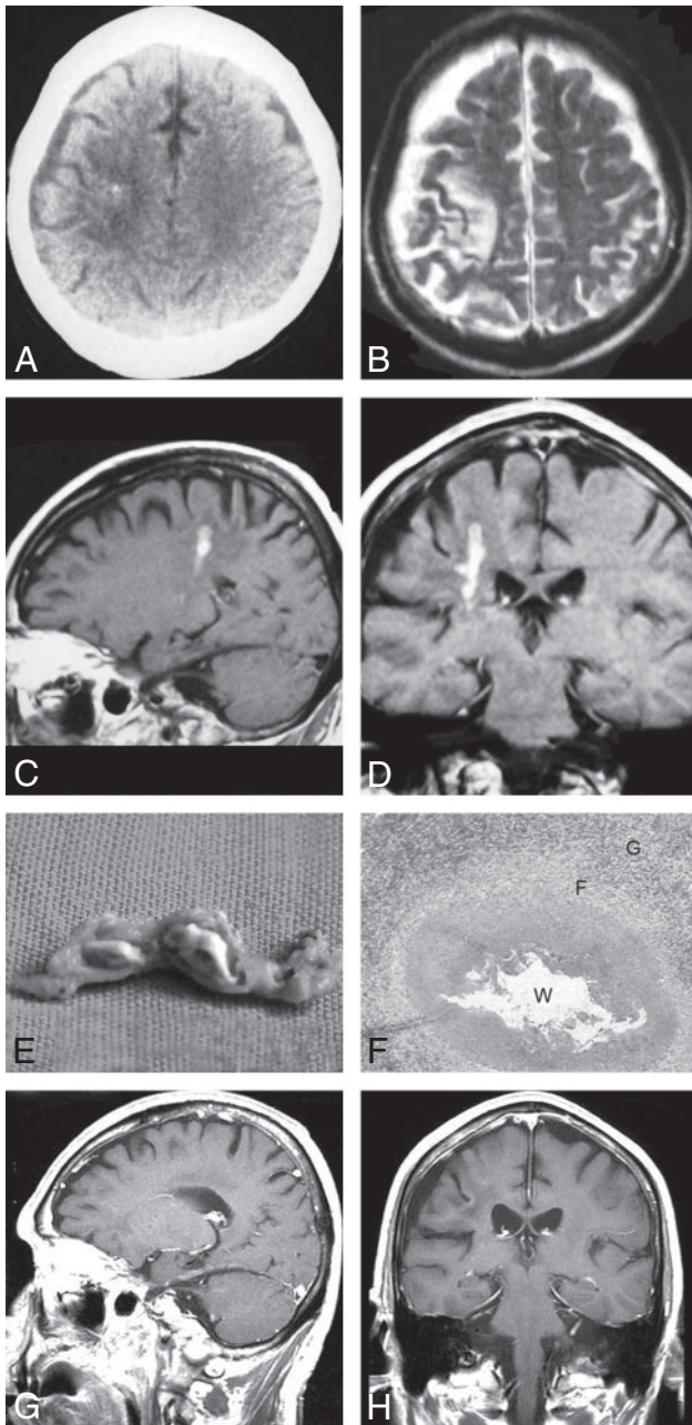
Fig 1. Case 1. Images of the brain of an 80-year-old man with a history of headache, seizure, and left hemiparesis for 2 years. A , Precontrast CT scan shows patchy area of hypoattenuation in the white matter of the right parietal lobe with a punctate calcification located centrally. B , Axial T2-weighted MR image of the same day shows hyperintense area and cortical atrophy in the right parietal lobe. However, calcification seen on CT image cannot be found on MR images. C–D , Sagittal and coronal postcontrast images show tunnel-shaped enhancement representing inflammatory granuloma. No ipsilateral ventricular dilation is seen. E , Postoperative gross photograph of resected specimen shows a degenerated worm of Spirometra mansoni surrounded by inflammatory granulomatous tissues. F , Photomicrograph of histologic specimen shows a removed degenerated worm ( W ) surrounded by collagen capsule ( C ) and peripheral inflammatory cells and gliosis ( G ) (H&E stain \times 40 ). G–H , Sagittal and coronal postcontrast images 1 year after a craniotomy in the same patient show lesions excised, with edematous area in the right parietal lobe.
